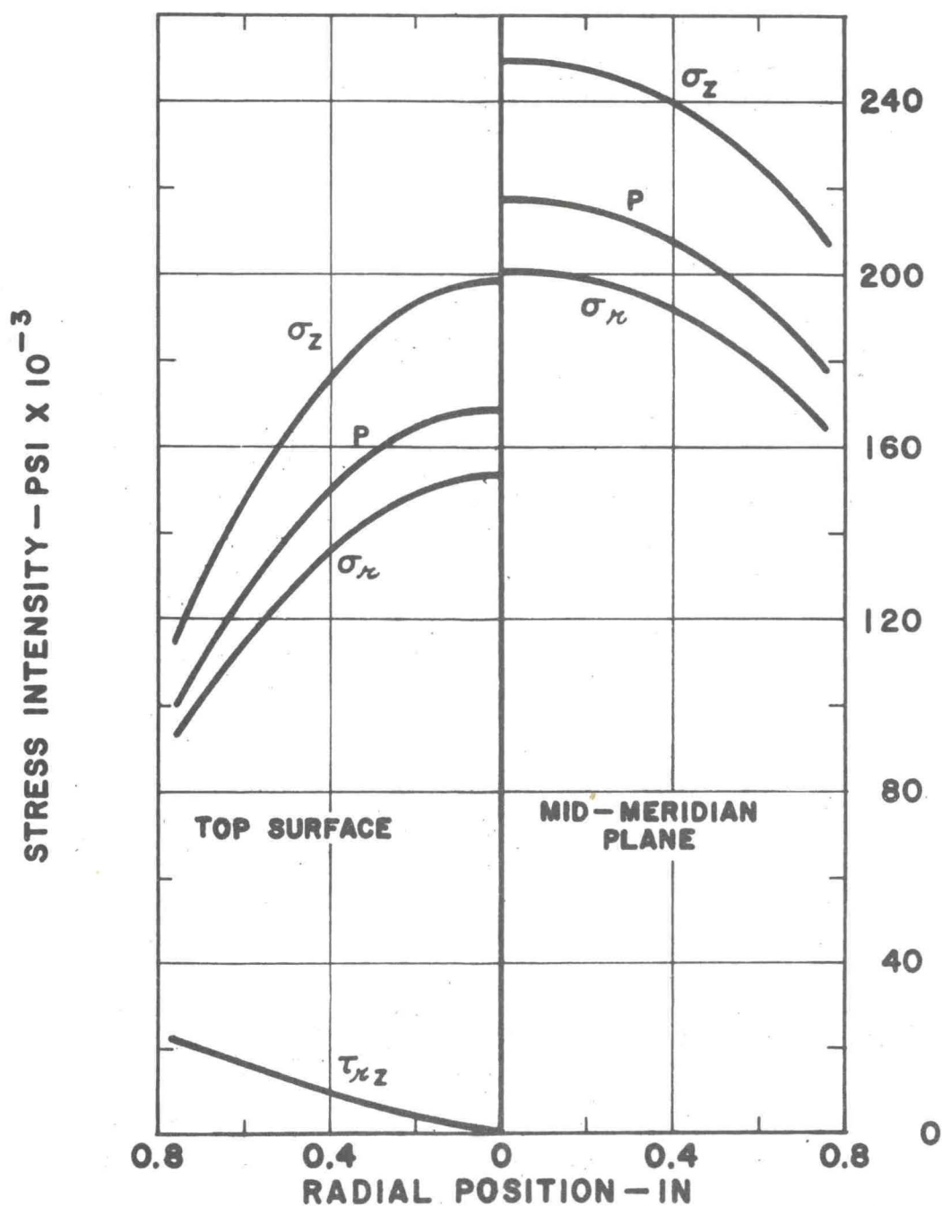
FIG. 14 STRESS DISTRIBUTION FOR 303 STAINLESS STEEL. CASE II - A R_c/R_0 = 1.012 .
